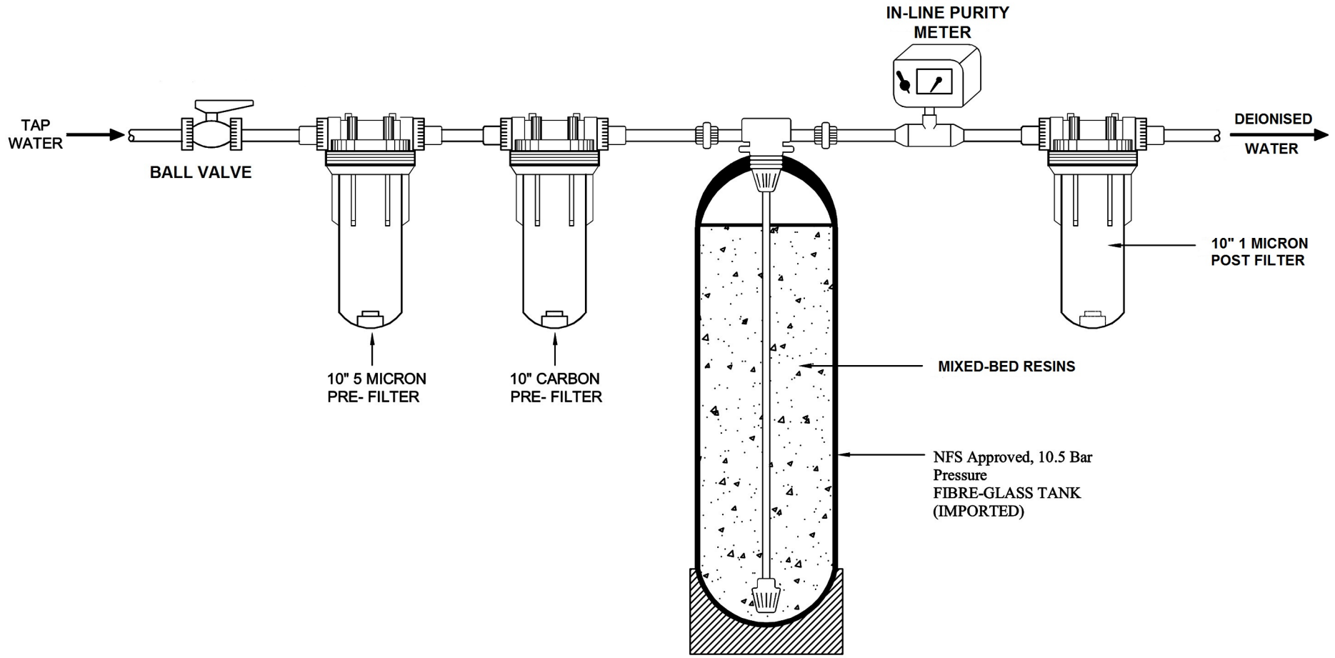
PORTABLE MIXED-BED DEIONIZER
